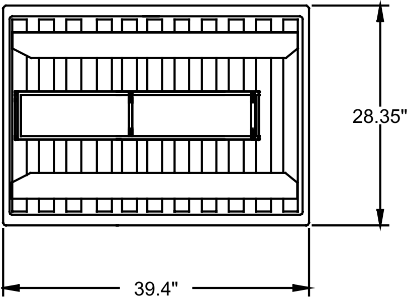
(RIGHT VIEW)
