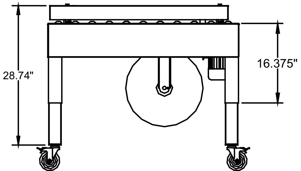
(RIGHT VIEW)
